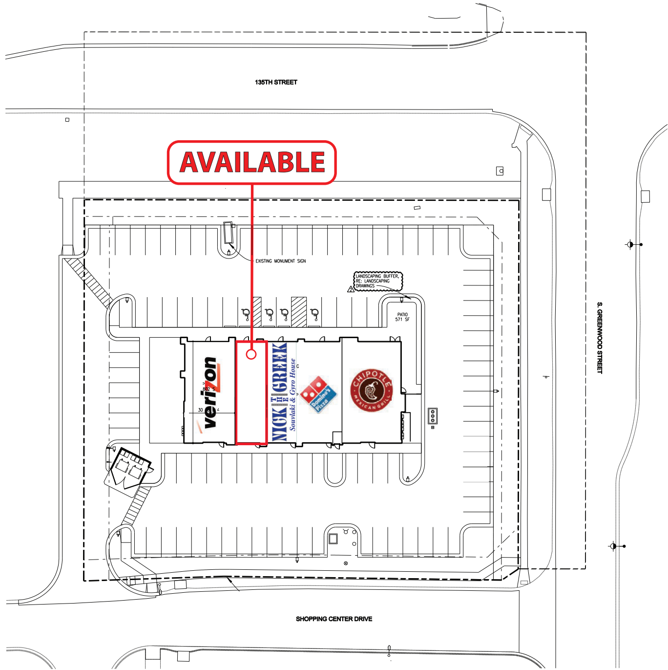
M1 ARCHITECTURAL SITE PLAN 1"=20'
